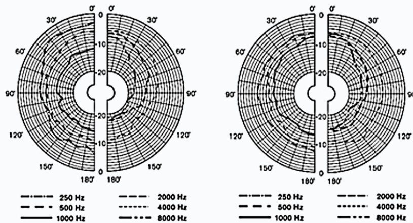
Vertical directivity pattern
