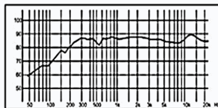
Freq.Response (dB SPL, 1W, 1m)
